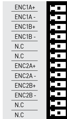
Pin arrangement
